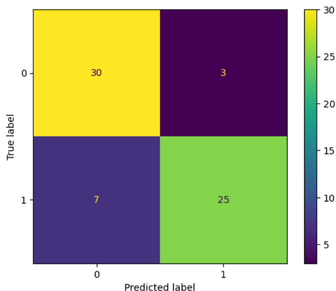
Figure 9. Confusion Matrix for Random Forest.
